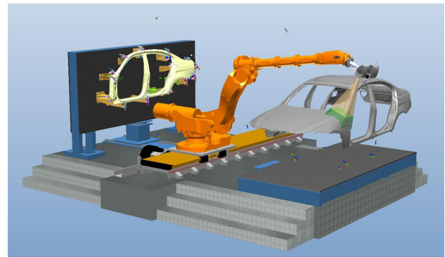
Figure 1. Industrial surface inspection cell
